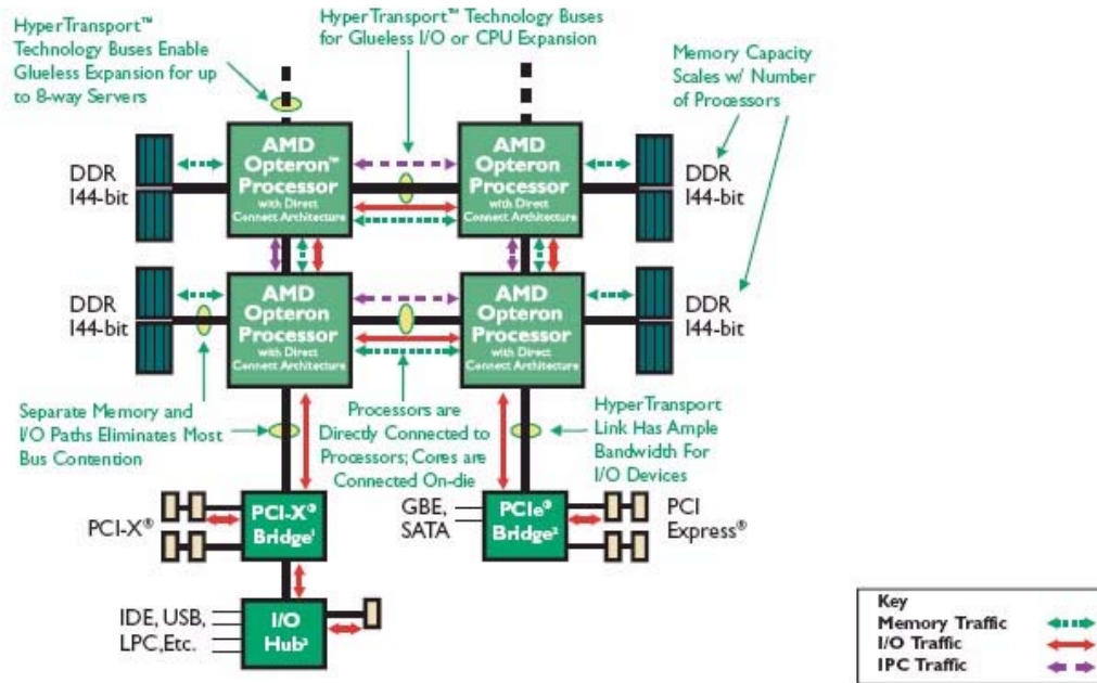
Figure 3. Diagram of an AMD Opteron processor-based 4P Server
